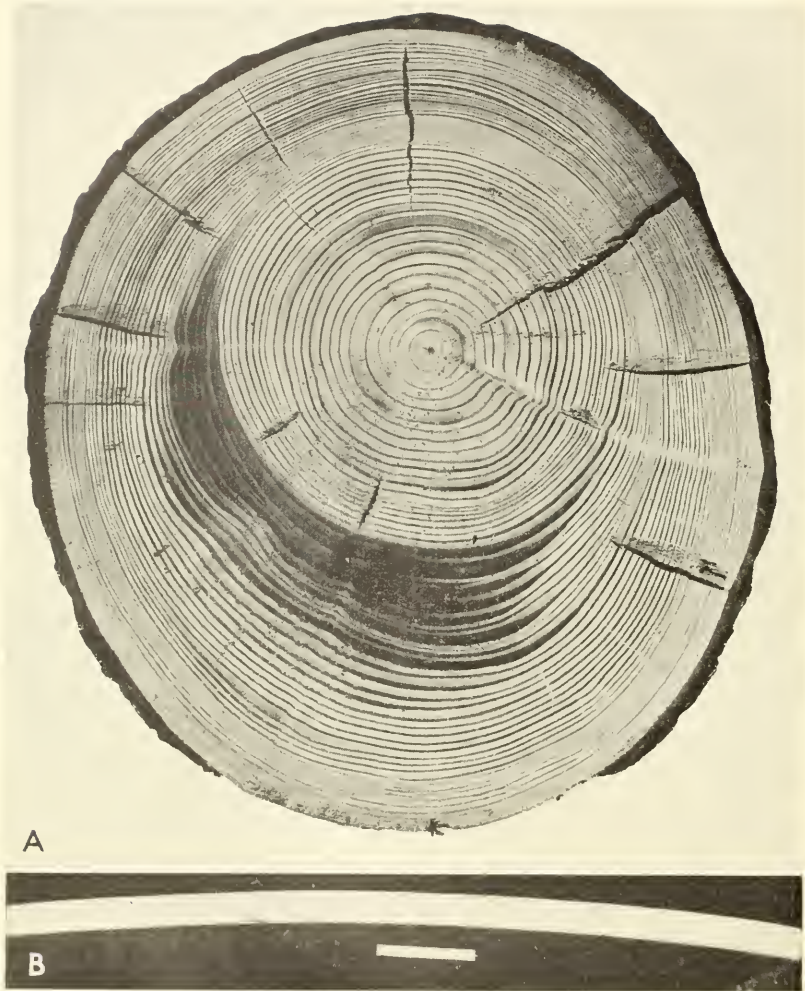
Compression wood: A, The dark, wide rings in the lower part of the cross section are compression wood; B, crook caused by the extreme longitudinal shrinkage of compression wood on the upper edge of a 2 by 4 inch stud. The 12-inch ruler indicates the length of the 8-foot stud
